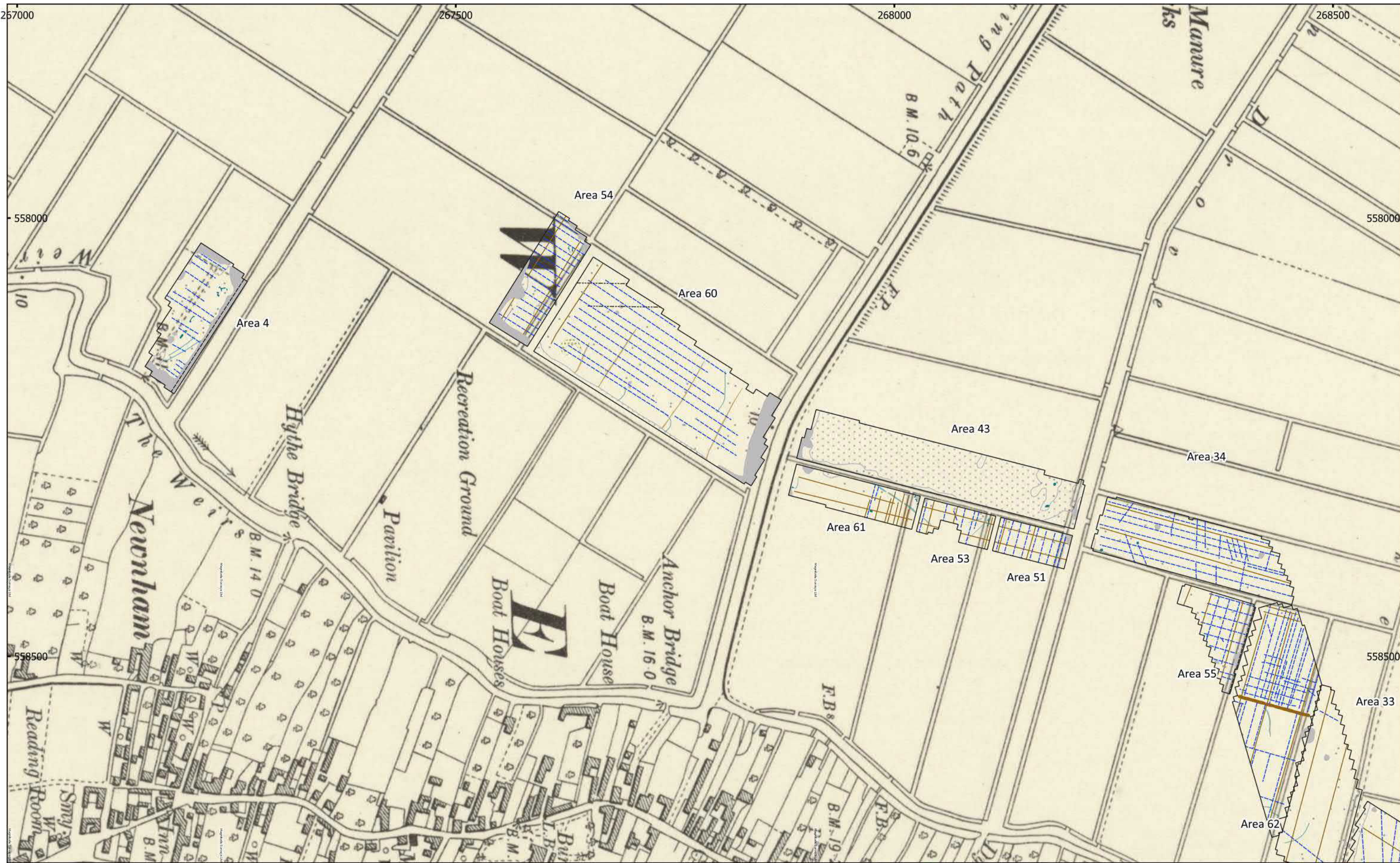
MSTL551 - Sunnica Energy Farm Reporting Zone H Figure H41 - Magnetic Interpretation Over Historic Maps (Overview) (West) 1:4,000 @ A3 Copyright Magnitude Surveys Ltd 2021 Contains historic maps: Ordnance Survey, 6" 2nd edition c. 1882-1913 © National Library of Scotland
